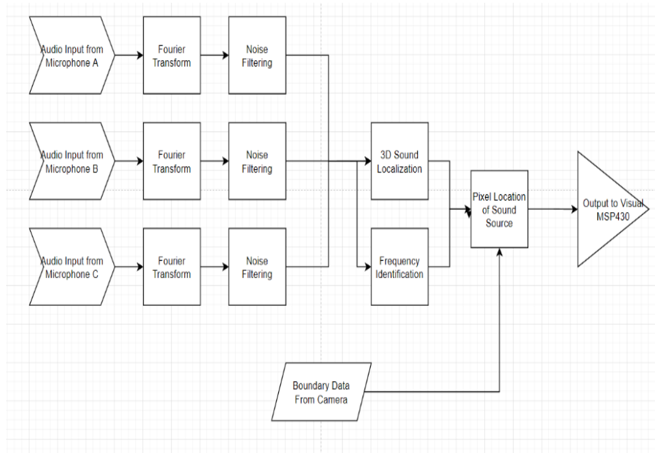
Figure 42: Audio Software Flowchart
