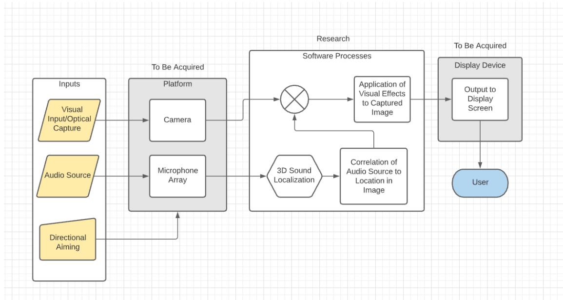
Figure 9: Device Block Diagram Overview
