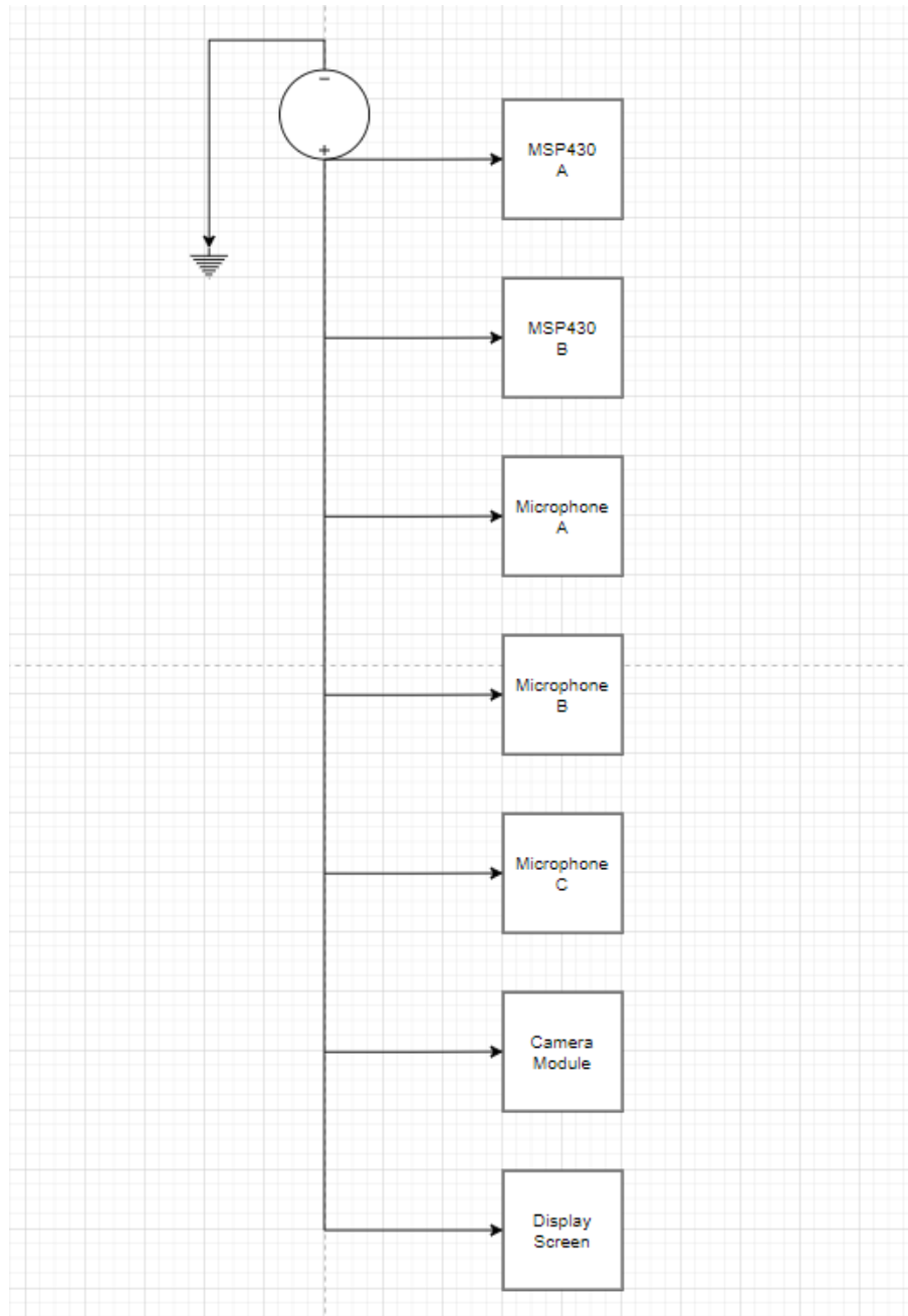
Figure 33: Power Supply Block Diagram
