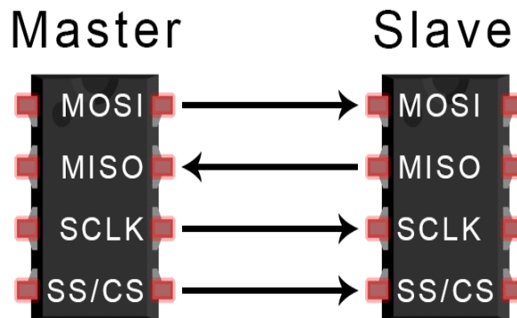
Figure 25: Simple SPI Configuration
