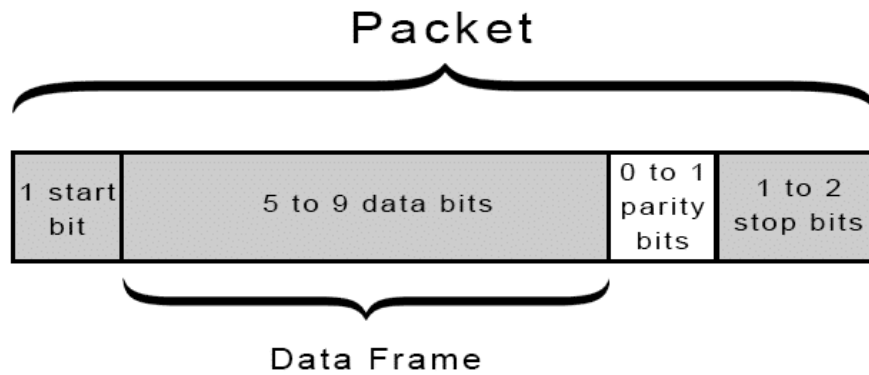
Figure 24: UART Data Packet
