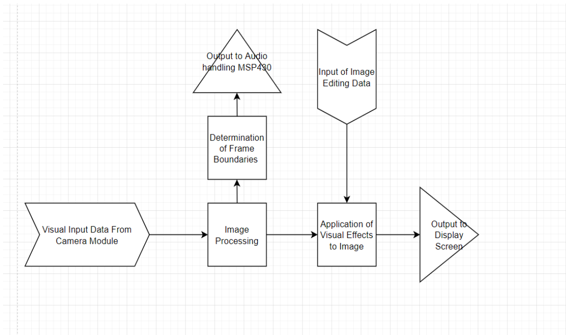
Figure 43: Visual Software Flowchart
