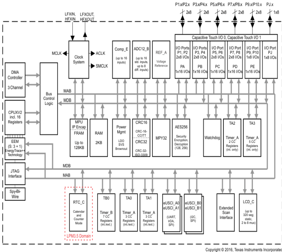
Figure 32: Block Diagram of MSP430
