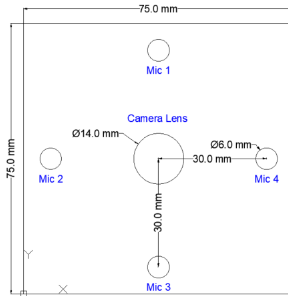
Figure 26: Front of Device
