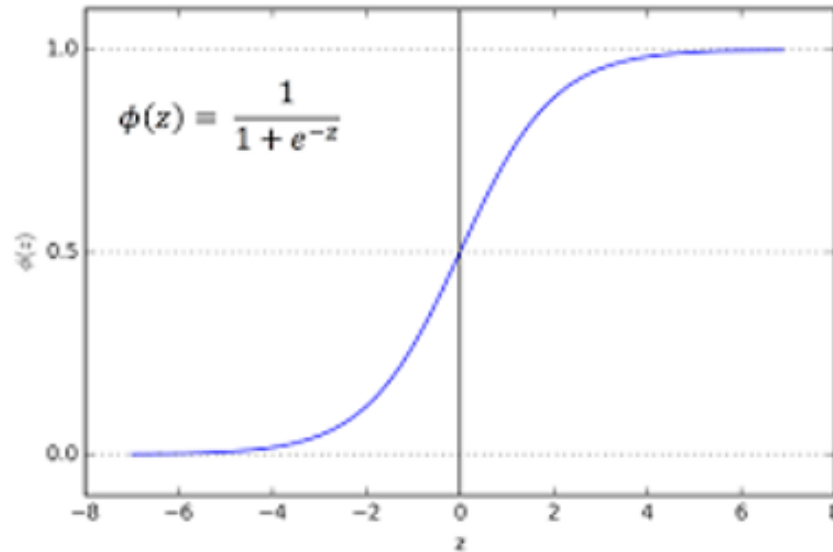
Figure 49: Sigmoid Function
