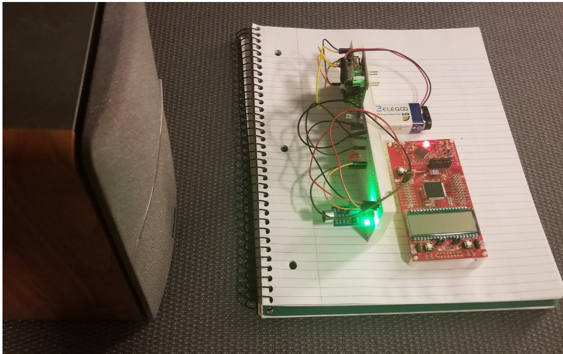
Figure 48: Testing of Blackbox Microphone Setup
